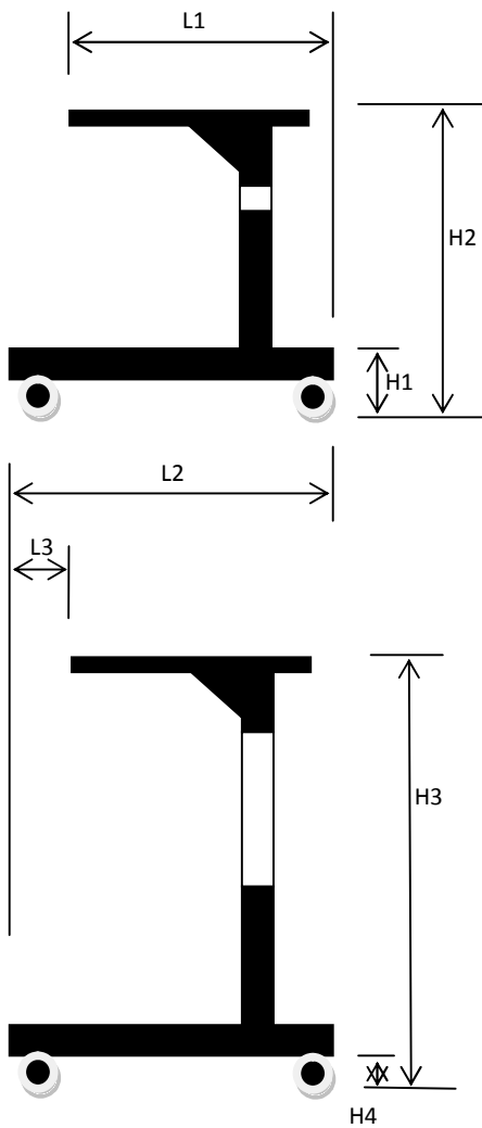
SIDE VIEWS
